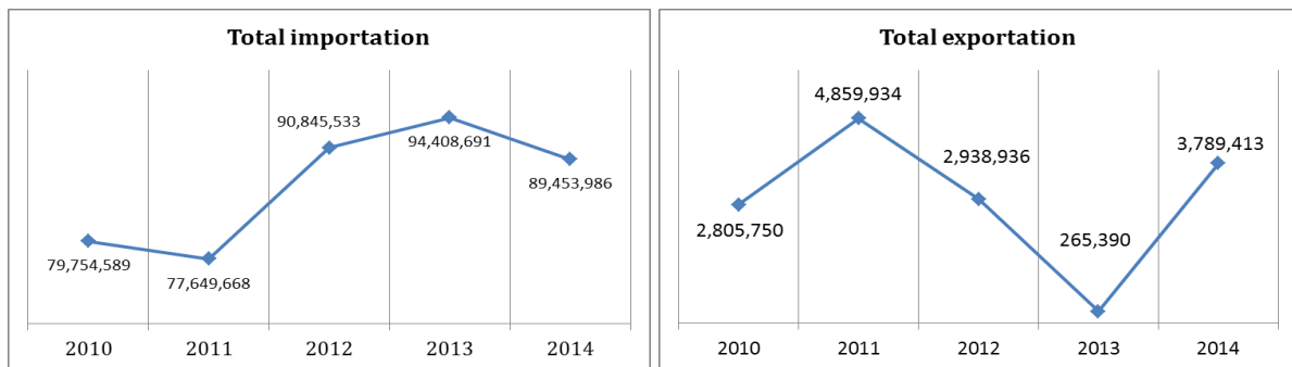
Figure 7.2: Electricity Exportation and importation (Kwh)
