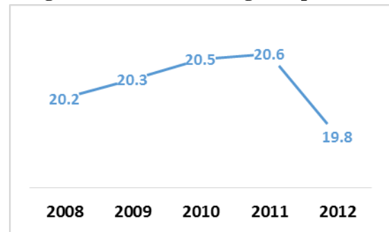
Figure 6.2: Annual average temperature
