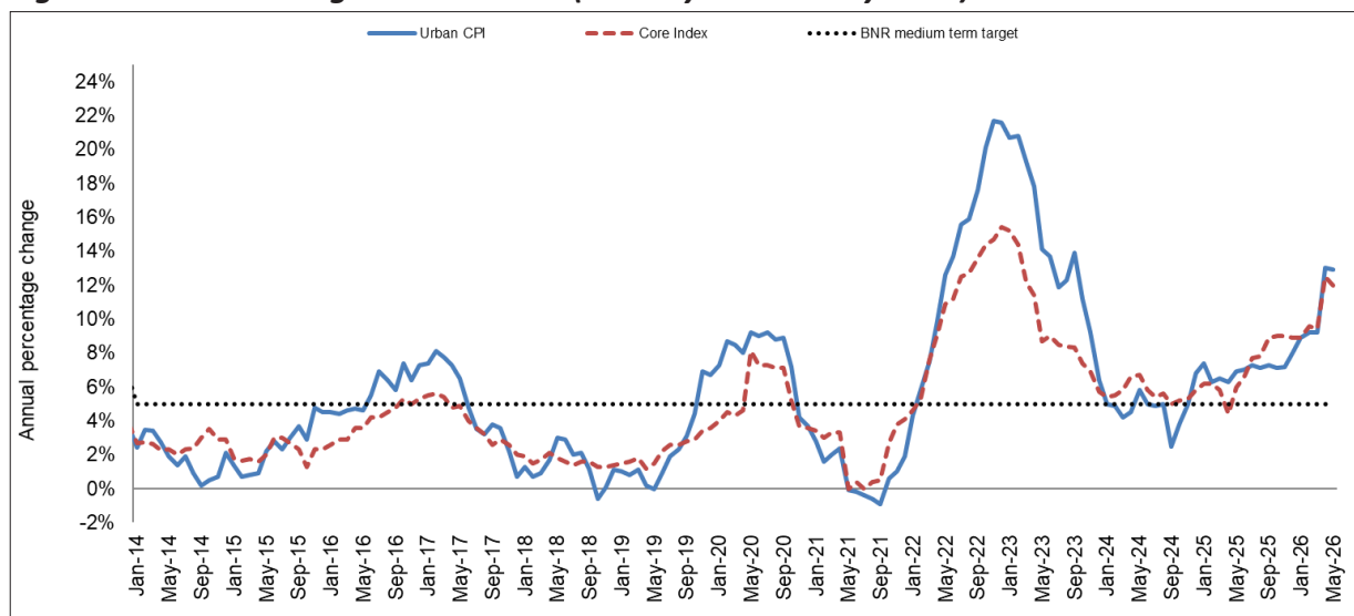
Figure 1: Annual changes in urban CPI (January 2014 – May 2026)
